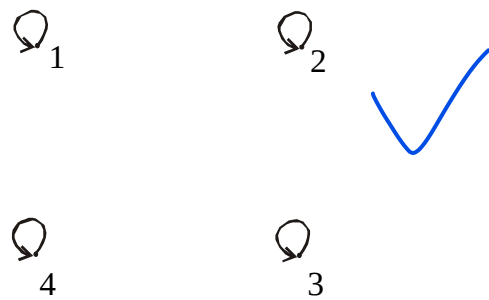
R_2 is symmetric
